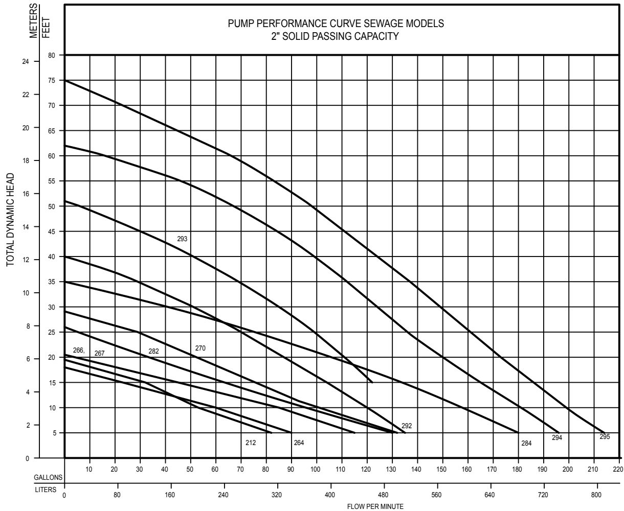
TOTAL DYNAMIC HEAD/FLOW PER MINUTE SEWAGE AND DEWATERING
